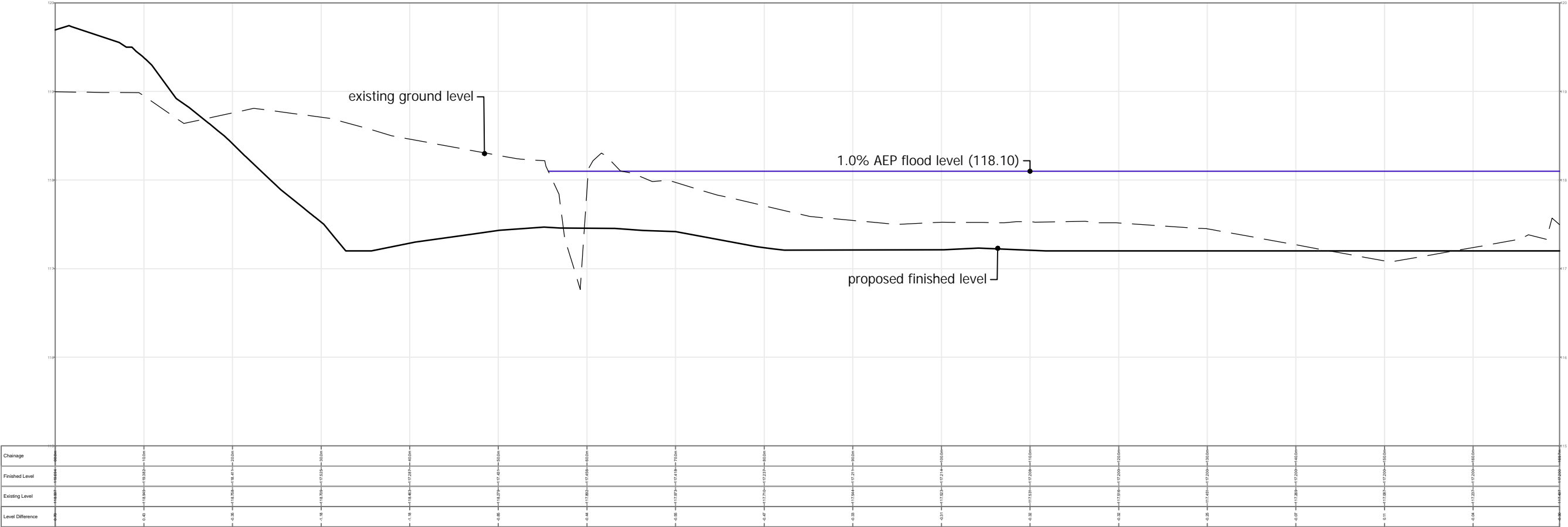
SECTION 1: LONGITUDINAL SECTION ALONG CENTRE OF COMPENSATORY STORAGE AREA Scale: 1:500H, 1:50V
