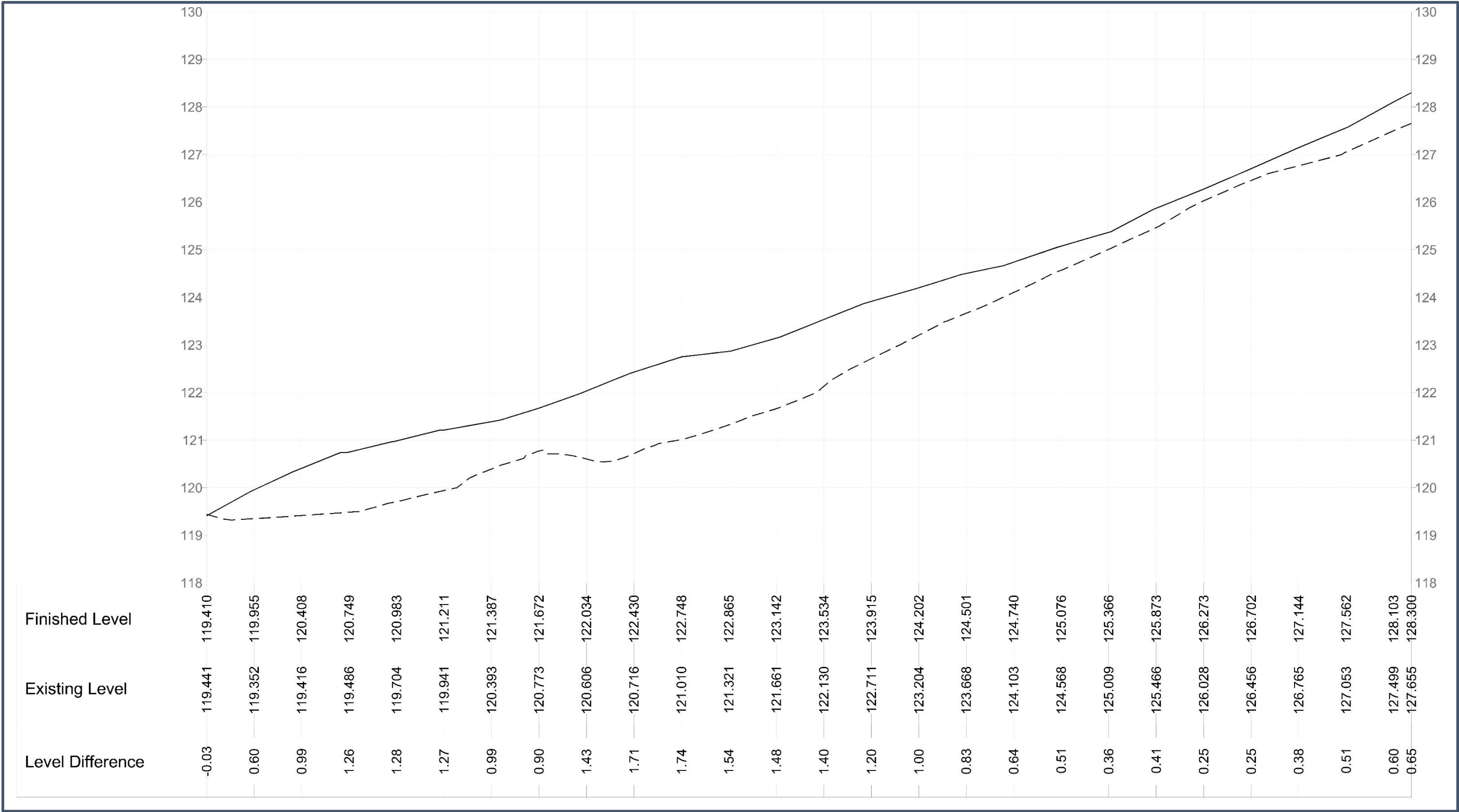
Figure 5.6a Profile through top of Raised Bank at East Boundary (Scale 1Horizontal:10 Vertical)
