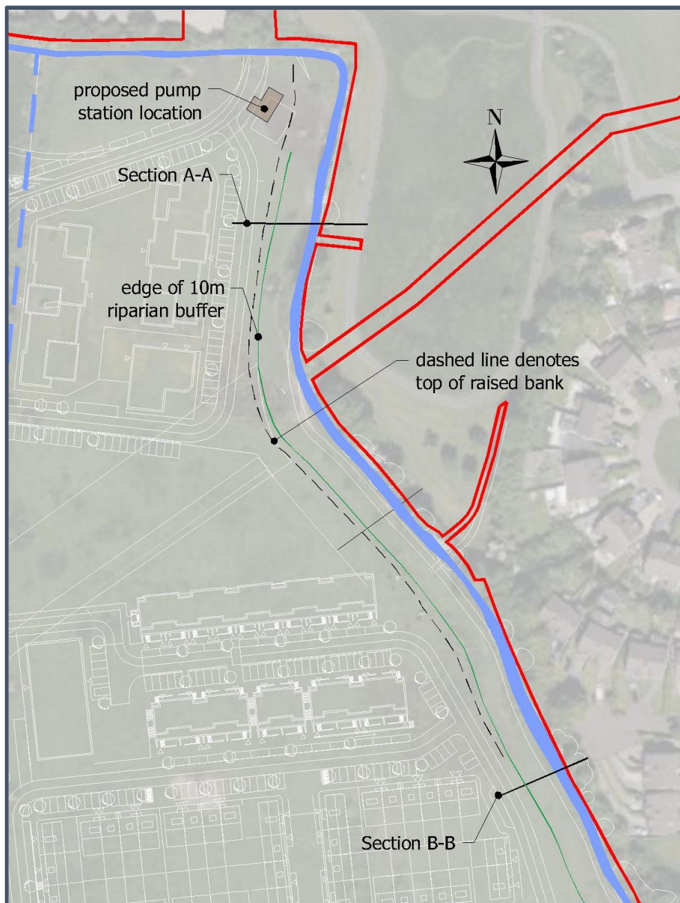
Figure 5.5 Raised Bank at East Boundary
