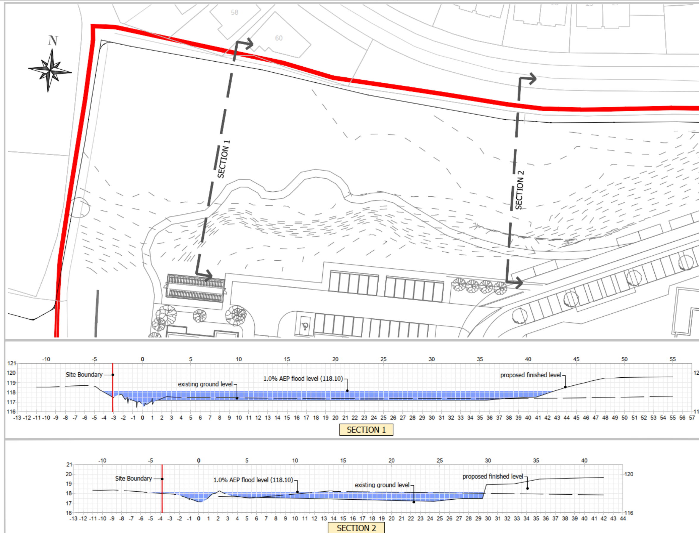
Figure 5.3 Plan and Typical Sections for Compensatory Storage Basin
