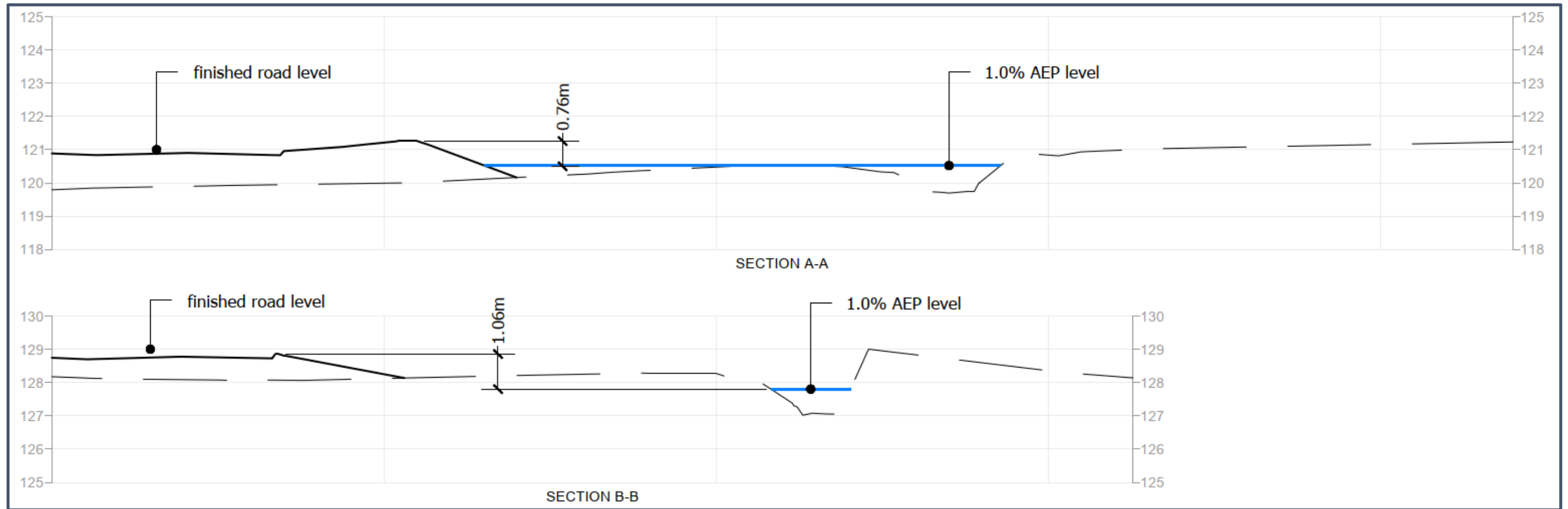
Figure 5.6 Sections showing 1.0% AEP flood level at Raised Bank
