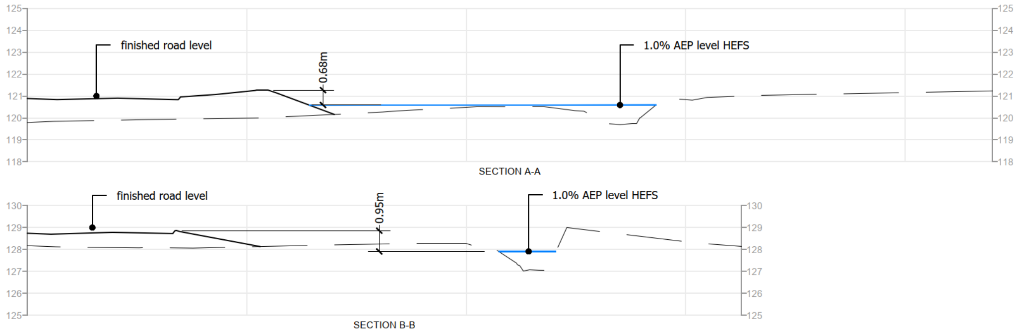
Figure 10-1 Sections at East Boundary in HEFS
