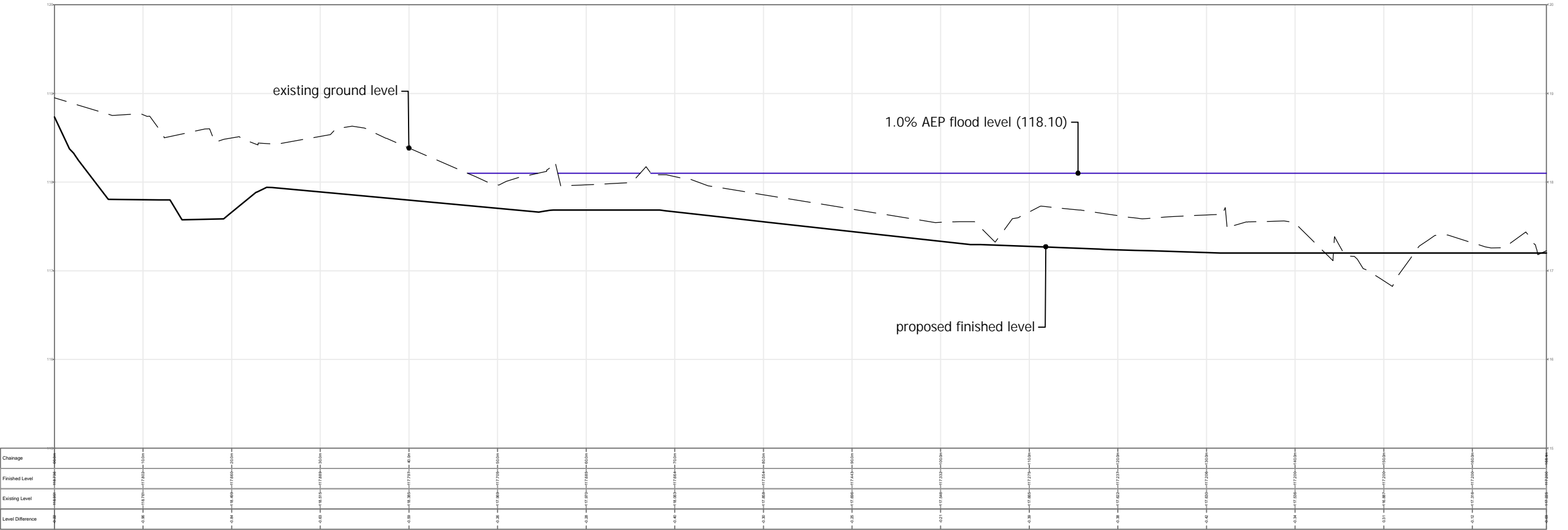
SECTION 2: LONGITUDINAL SECTION WITHIN COMPENSATORY STORAGE AREA ALONG EDGE OF CORBALLY STREAM Scale: 1:500H, 1:50V
